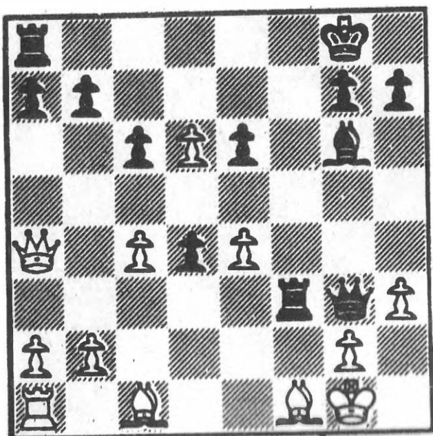
39 After 19 Bf1
